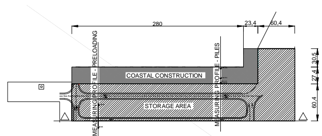
Figure 1 Plan view of the container terminal.
