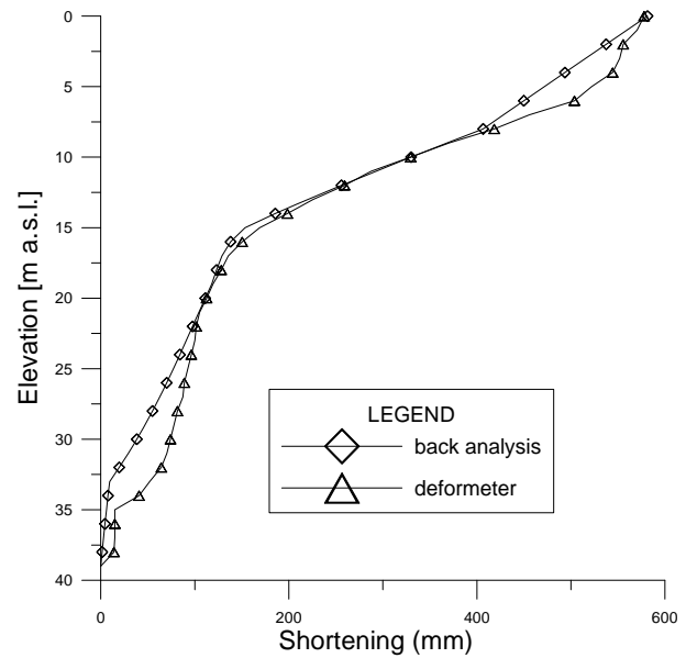
Figure 9 Soil settlement by layers in vertical deformer, and according to back analyses after 90 days of preloading.
