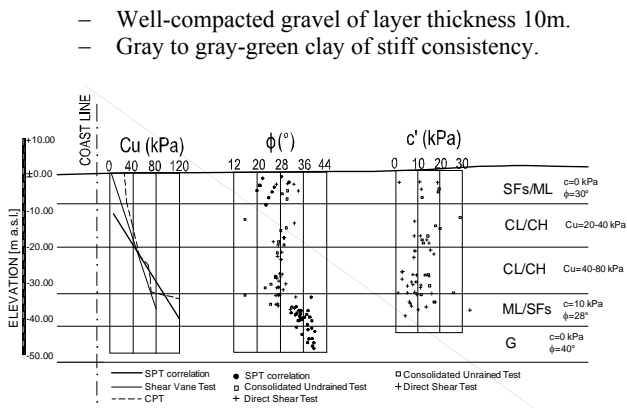
Figure 2 Geotechnical soil profile with performed in-situ exploratory works and laboratory tests.
