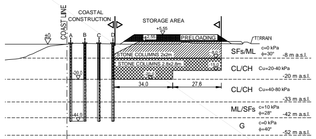
Figure 5 Construction phase II: execution of piles from the coast on previously prepared terrain.
