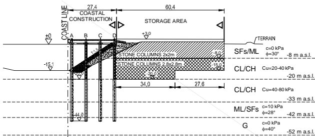
Figure 7 Construction phase IV: construction of coastal structure over piles.
